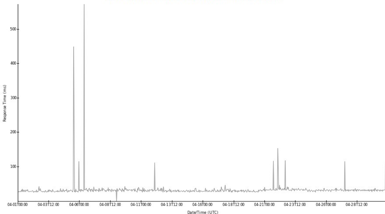
EPP Service IPv4 Uptime Report (obtained from Pingdom)
